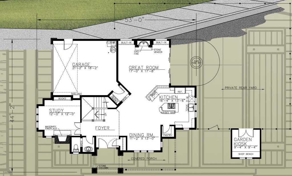
1213 ft 2 MAIN
