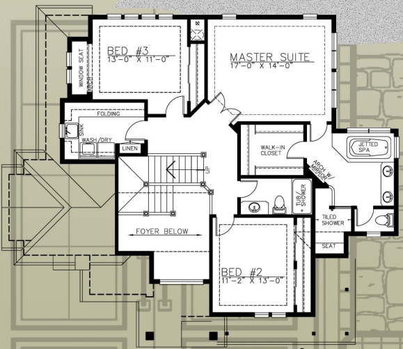
1191 ft 2 UPPER
