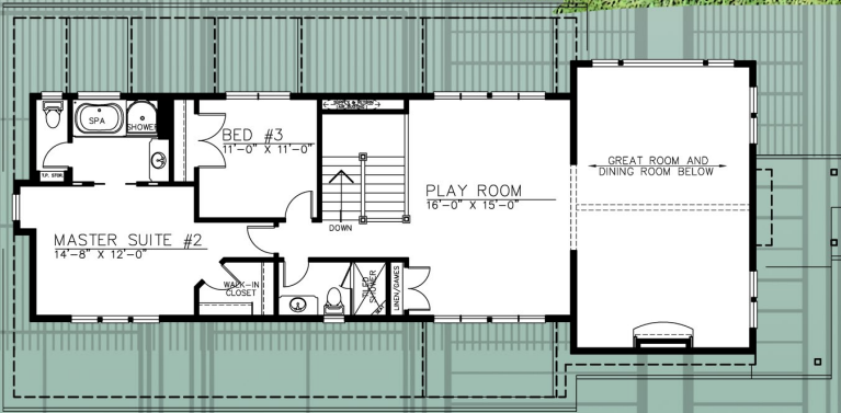
976 ft 2 UPPER
