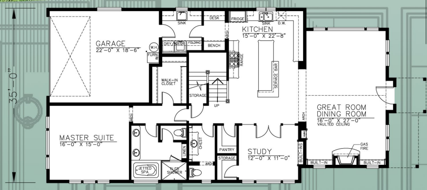
1863 ft 2 MAIN
